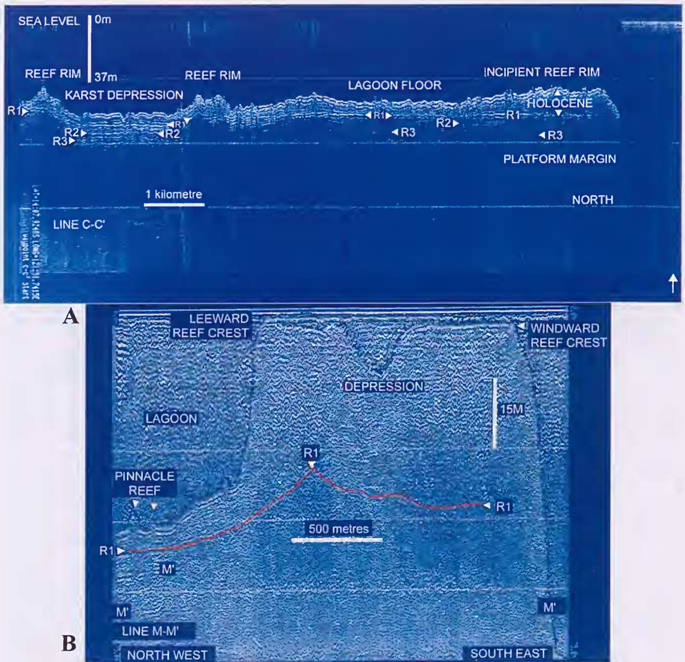
Figure 5. Seismic (boomer) architecture of Scott Reef platform (see Fig. 4 for location). A) Section C-C' of South Reef lagoon showing seismic discontinuities and karst depression. Three unconformities can be identified: R1, R2 and R3. R1 corresponds to the Last Interglacial (top MIS 5e) surface, underlain by MIS 7 and 9. B) South Reef boomer profile M-M' across reef crest (see Fig. 4 for location). Note presence and elevation of R1 beneath the Holocene reef crest (from Collins 2002).
